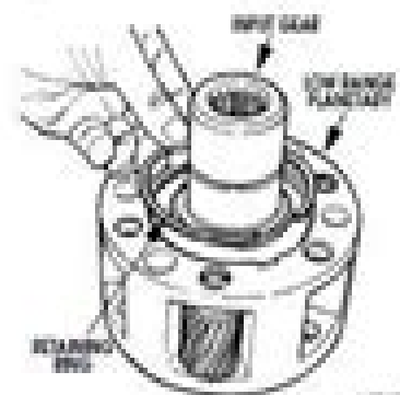
Figure 6-189 Input gear lock ring removal
