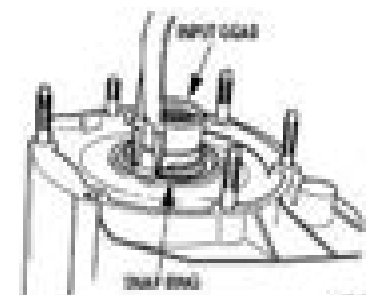
Figure 6-188 Input gear retaining ring removal
