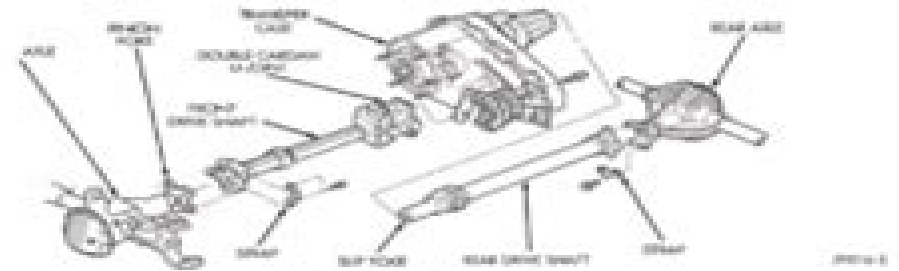
Fig. 1 Propeller Shaft 4J
