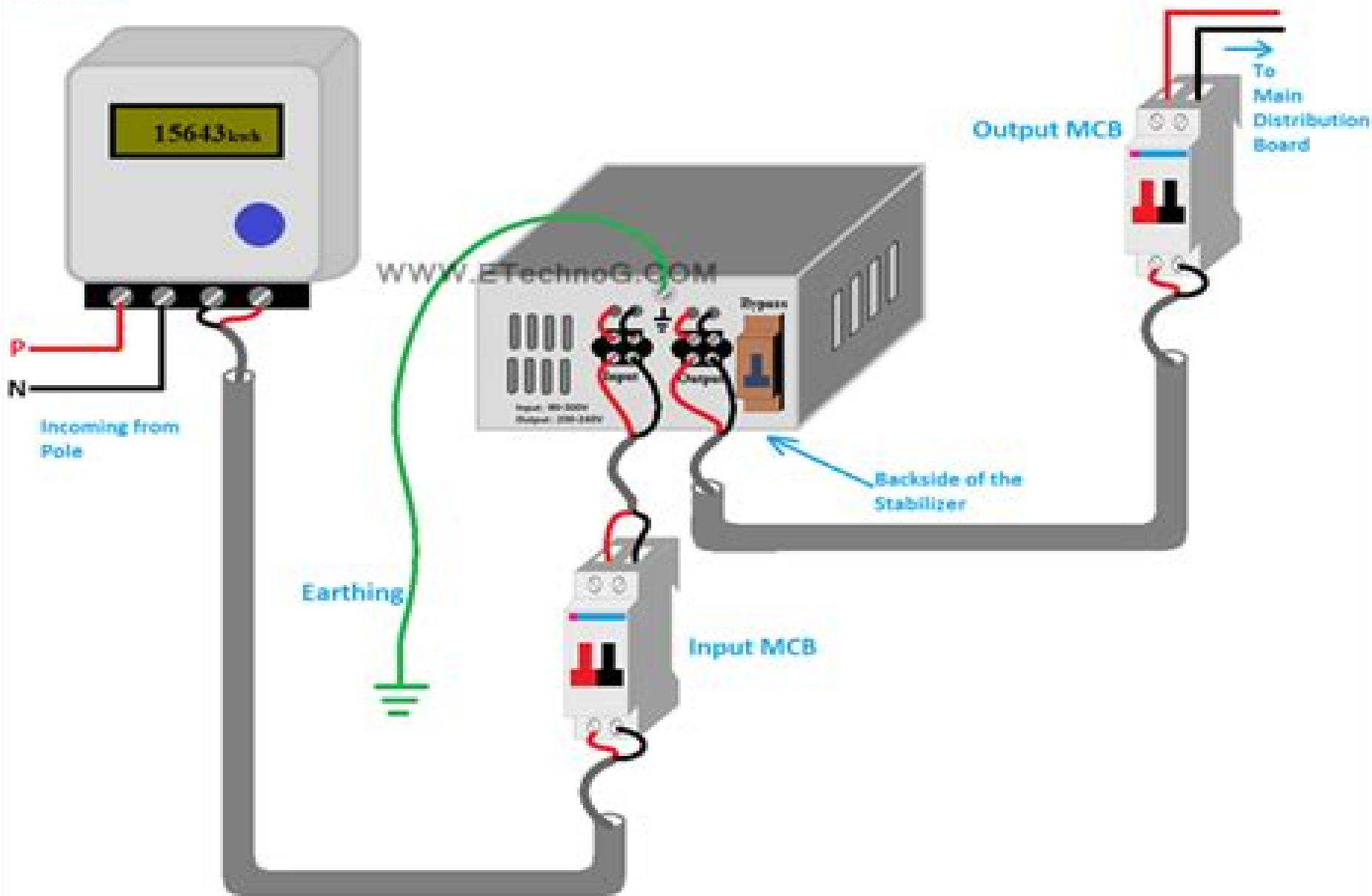
Stabilizer Connection Diagram for Home
