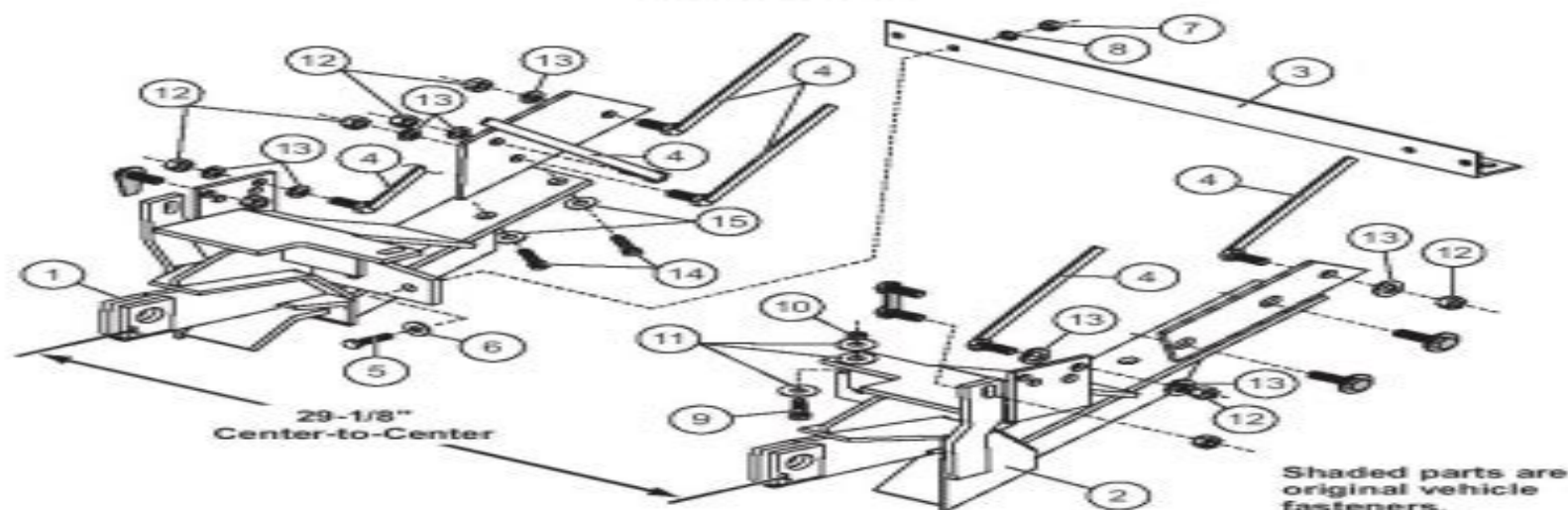
7157 Mount Kit
