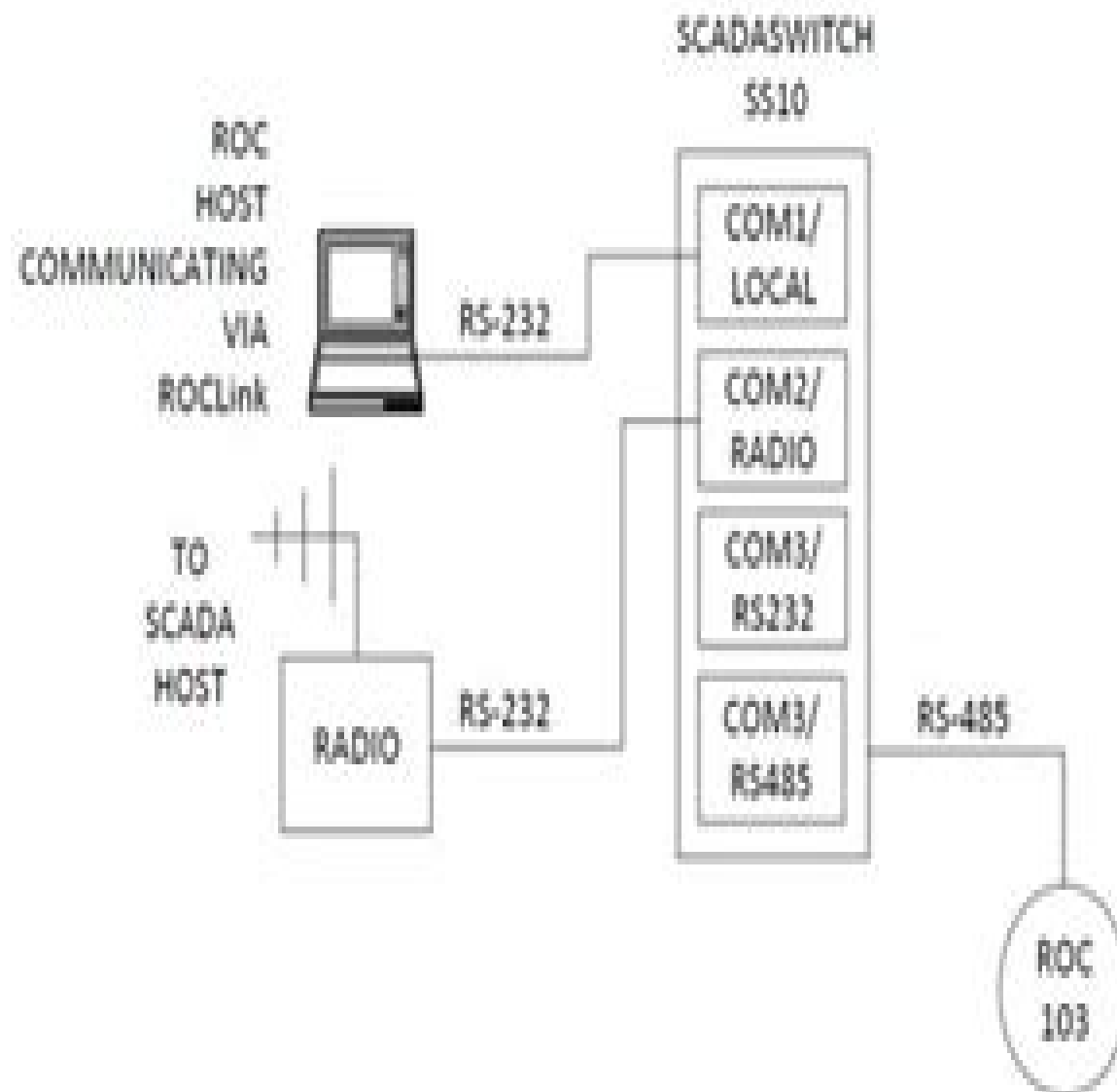
Simultaneous SCADA Polling and Fisher ROC FloBoss Diagnostics using SS10
