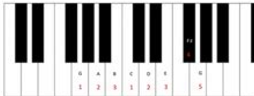
G major
