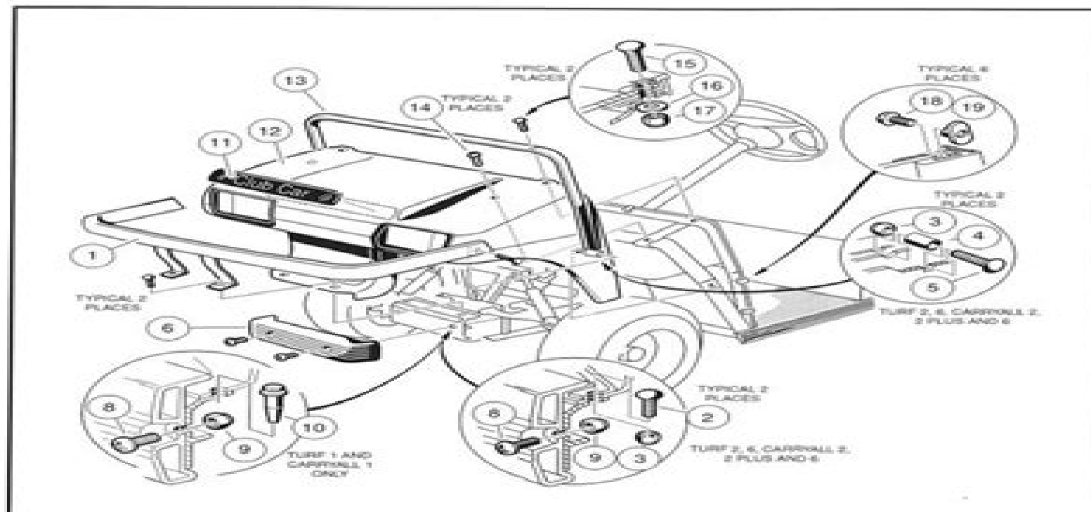
Figure 4-1 Front Body Assembly
