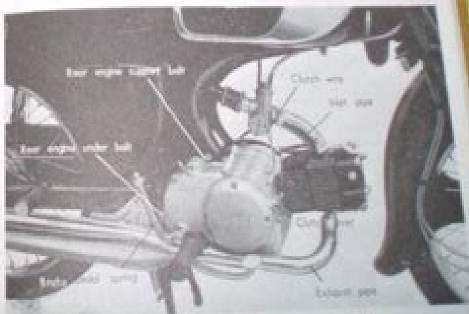
All items that must be removed before removing engine, Step 25.
