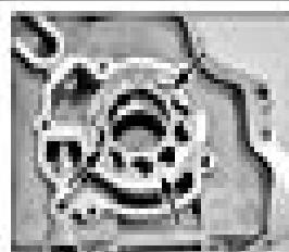
1.6 Clutch master cylinder - removal
