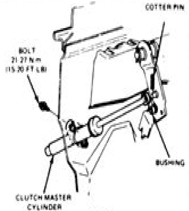
VIEW Z
