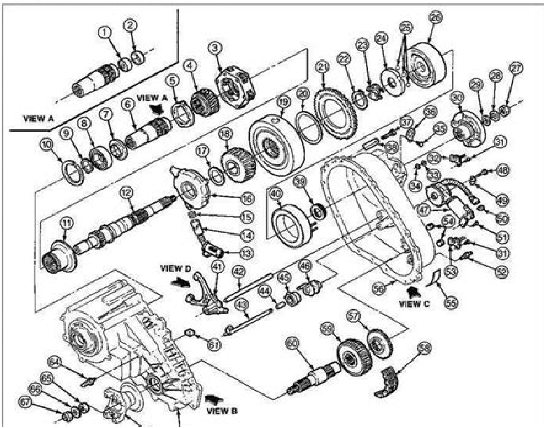
Transfer Case, 44-05 Control Trac, Disassembled View
