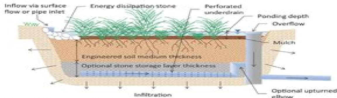
Figure 1. Cross-section view.
