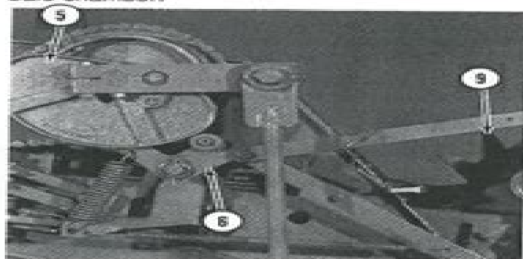
Figure MNT-61. Knotter Trip Arm Adjustment
