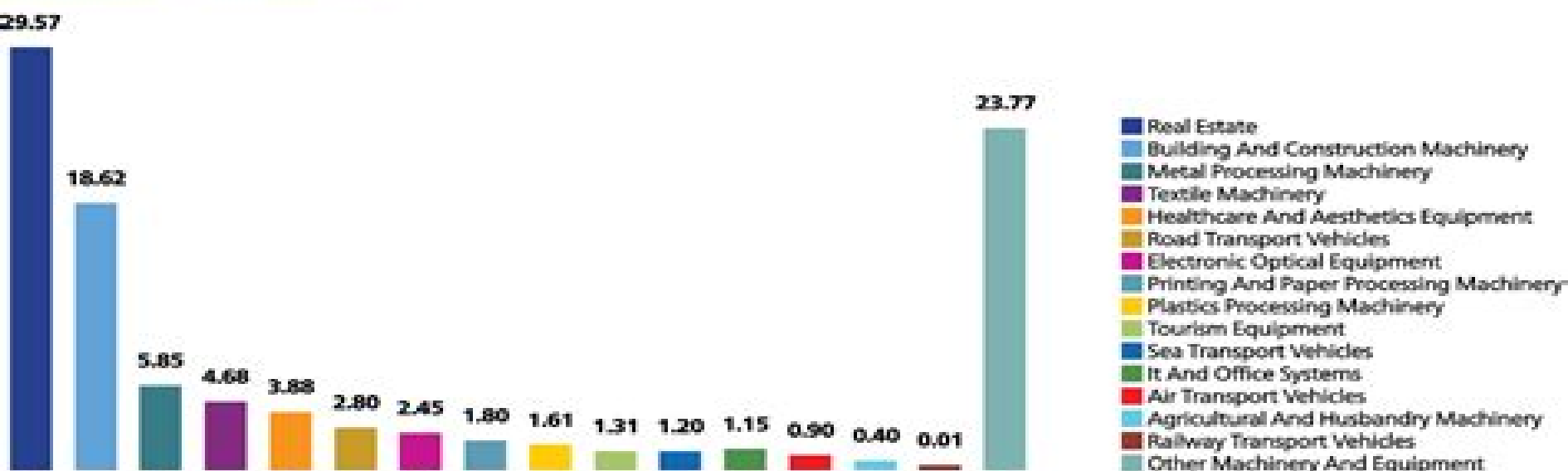
2018 EQUIPMENT DISTRIBUTION (%)
