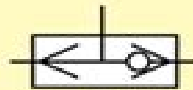
Shuttle Valve
