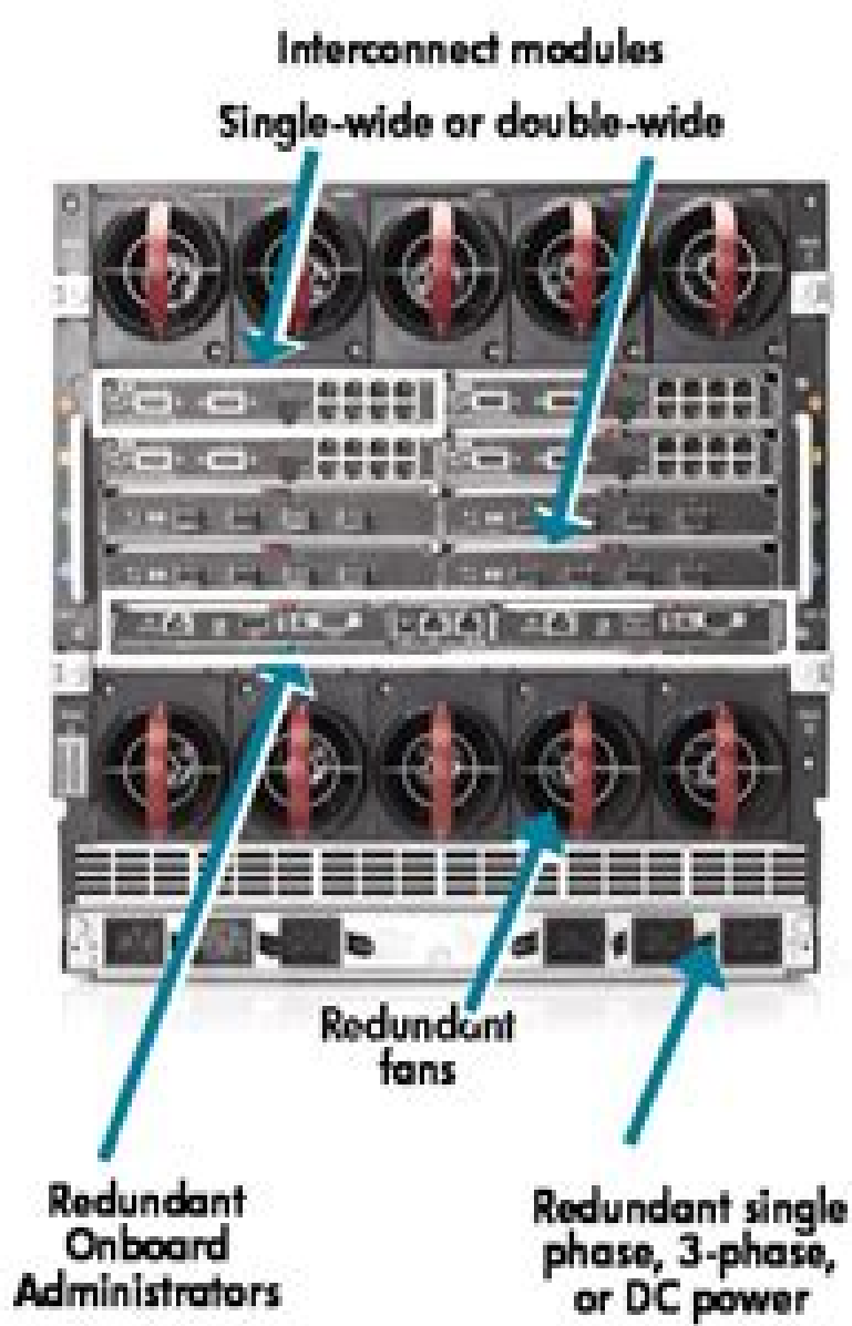
c7000 enclosure - back
