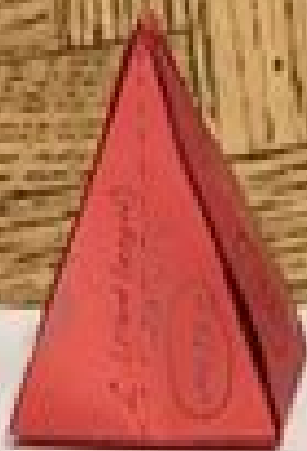
Square Pyramid
