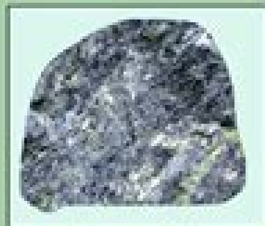
Blue schist
