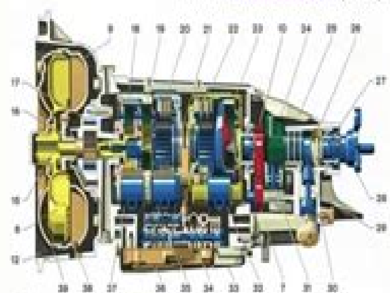
Fig. 1 4-speed transmission with fluid coupling
