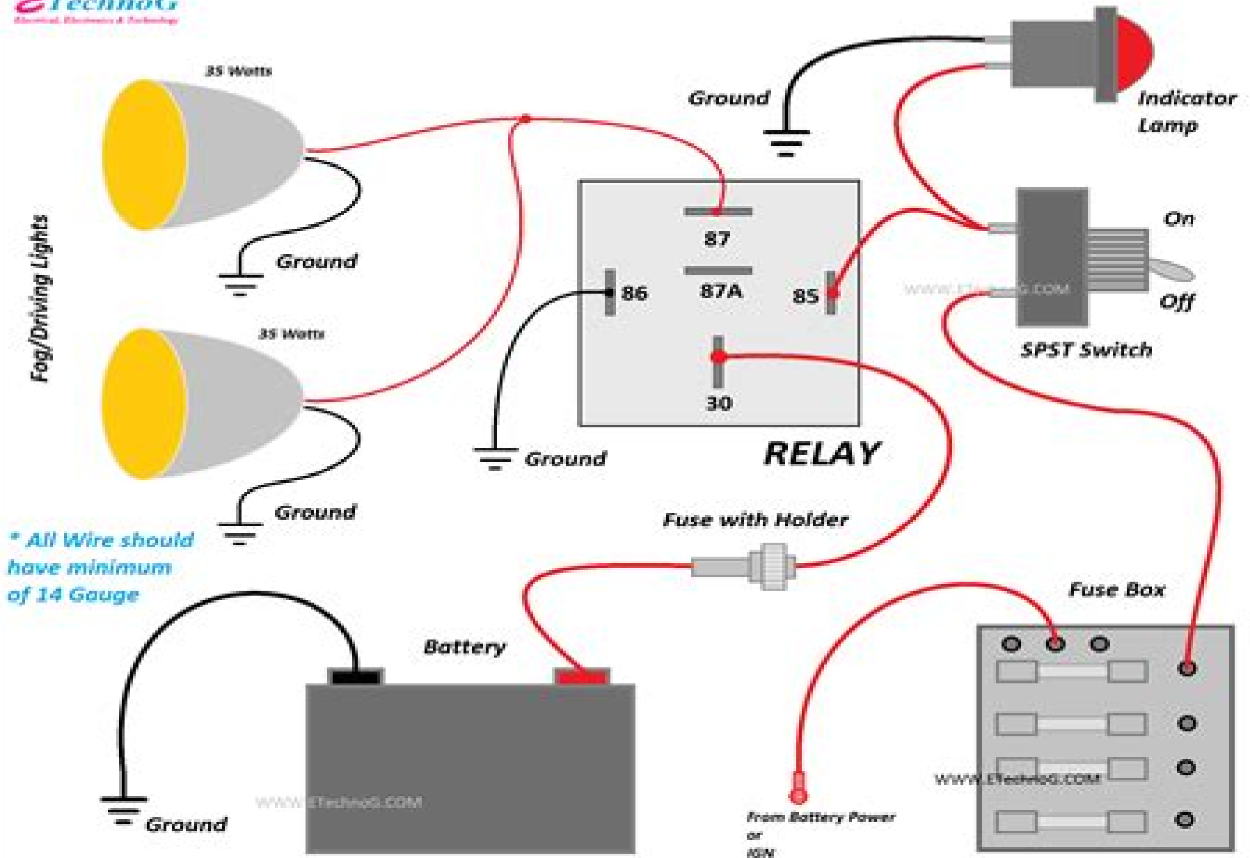
Fog Light Wiring and Connection Diagram with Relay and Switch
