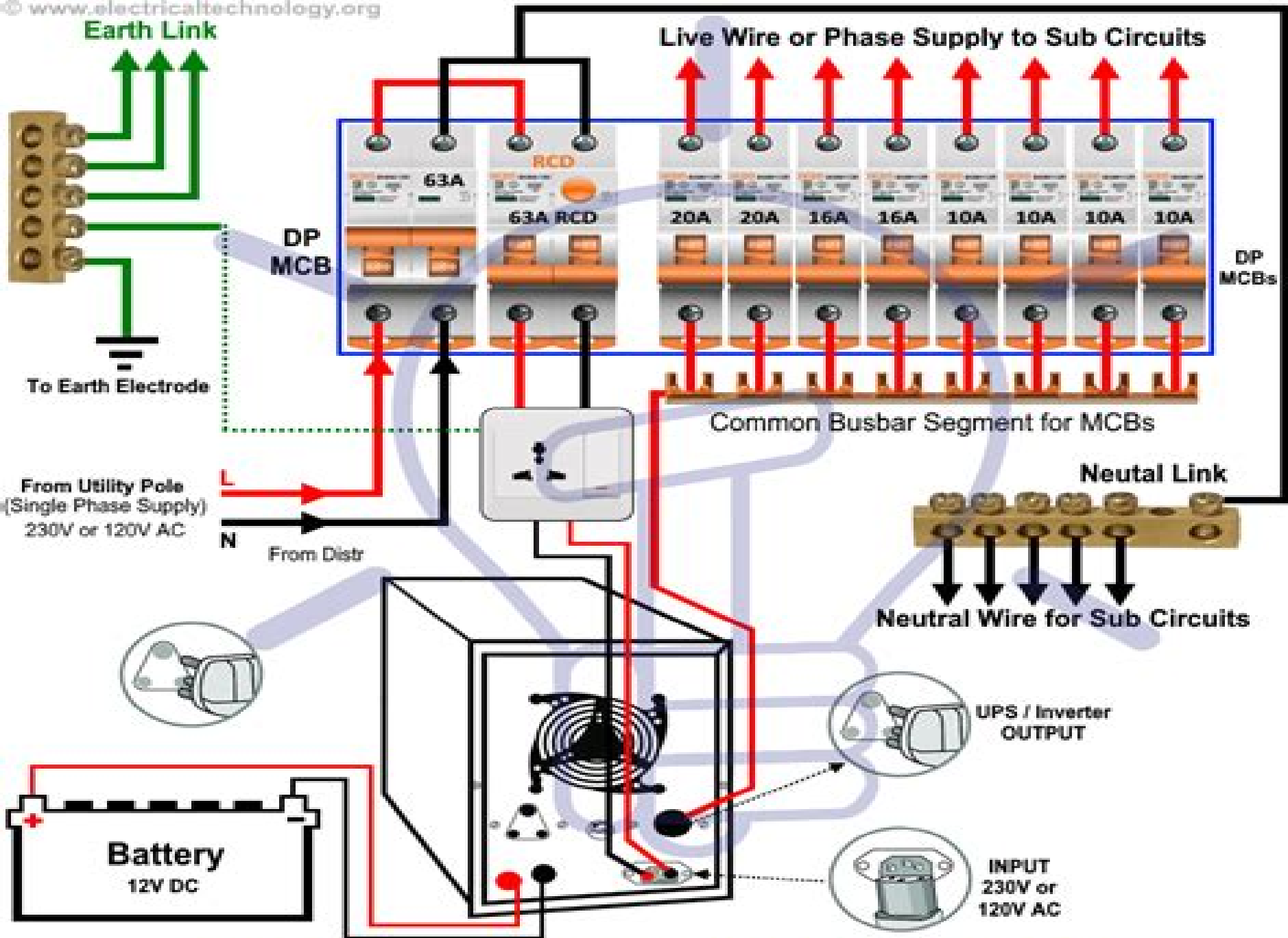
How to Wire UPS / Inverter to the Home Supply ?
