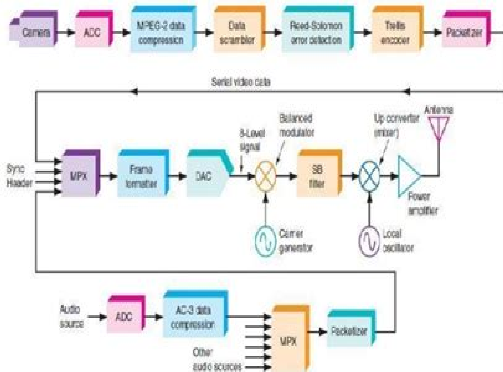
Figure 23-27 HDV transmitter.
