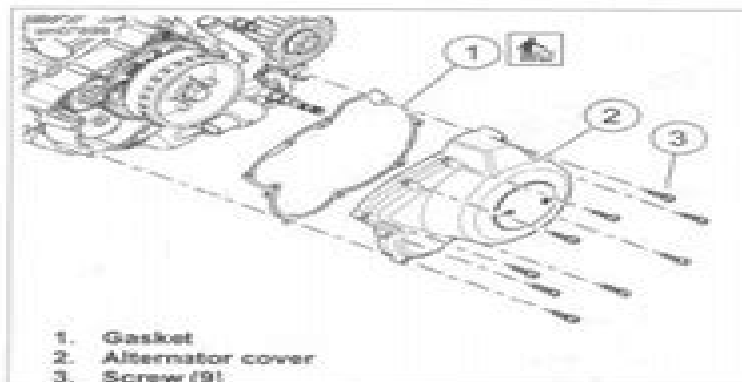
Figure 4-33. Alternator Cover
