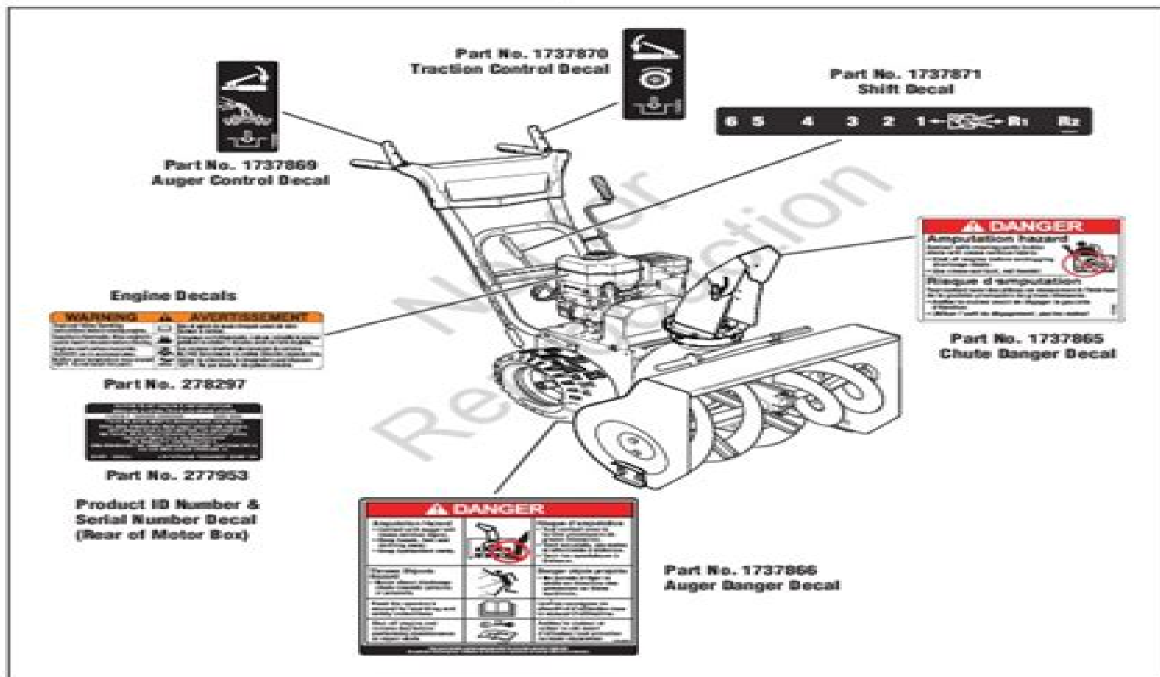
Safety Decals
