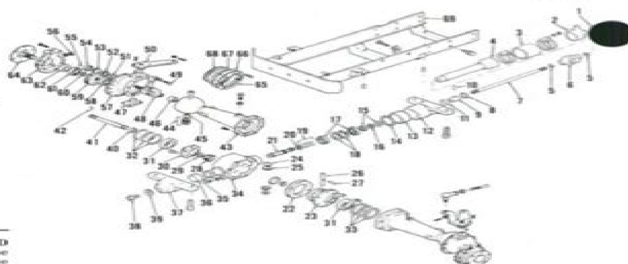
Fig. 7—Exploded view of front wheel drive axle used on 1100 and 1200 models.
