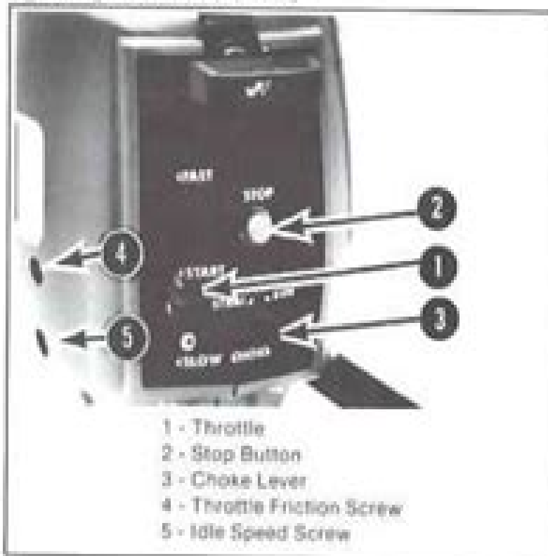
Fig. 9. Engine Controls (Model 2)
