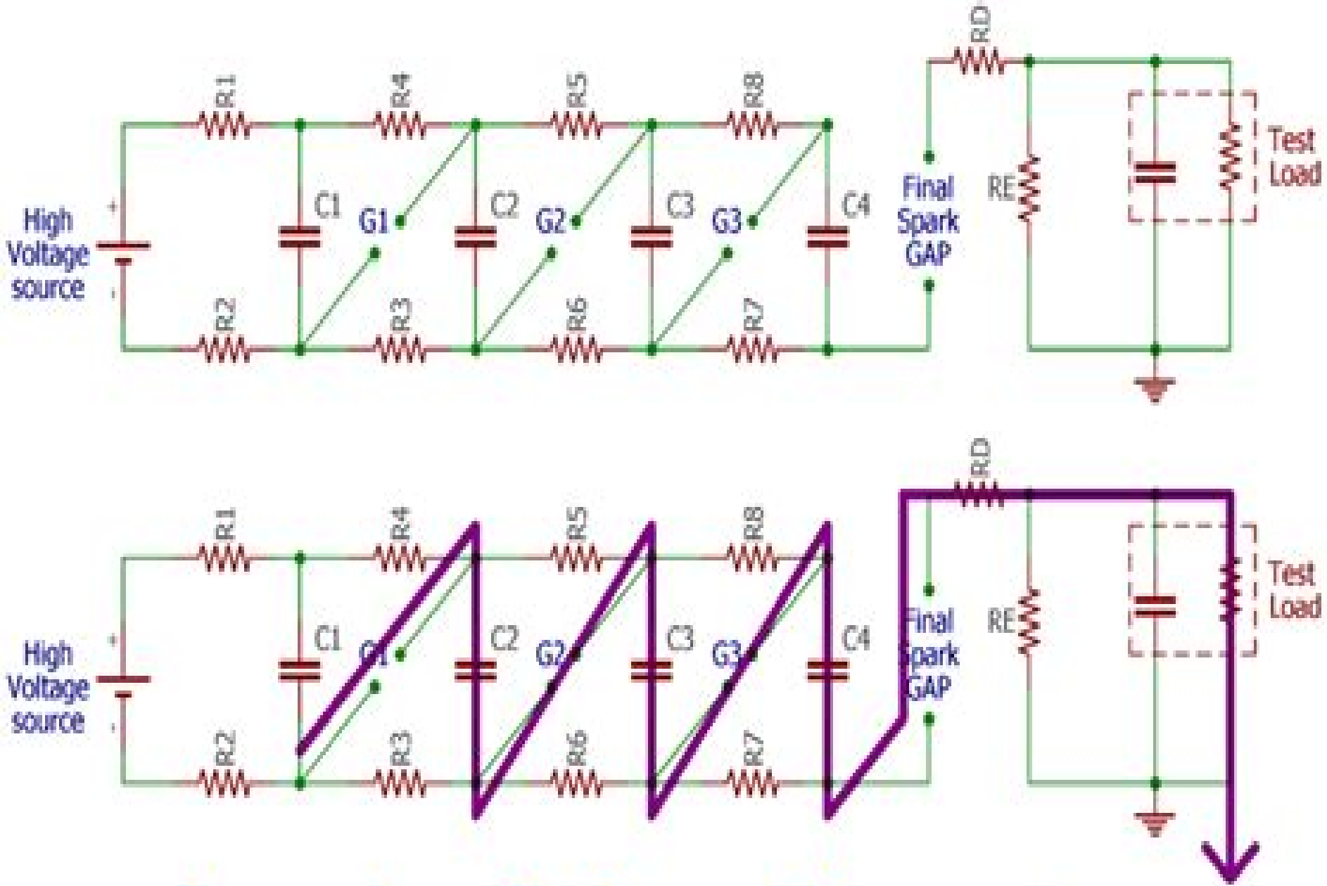
Impulse Voltage Generator
