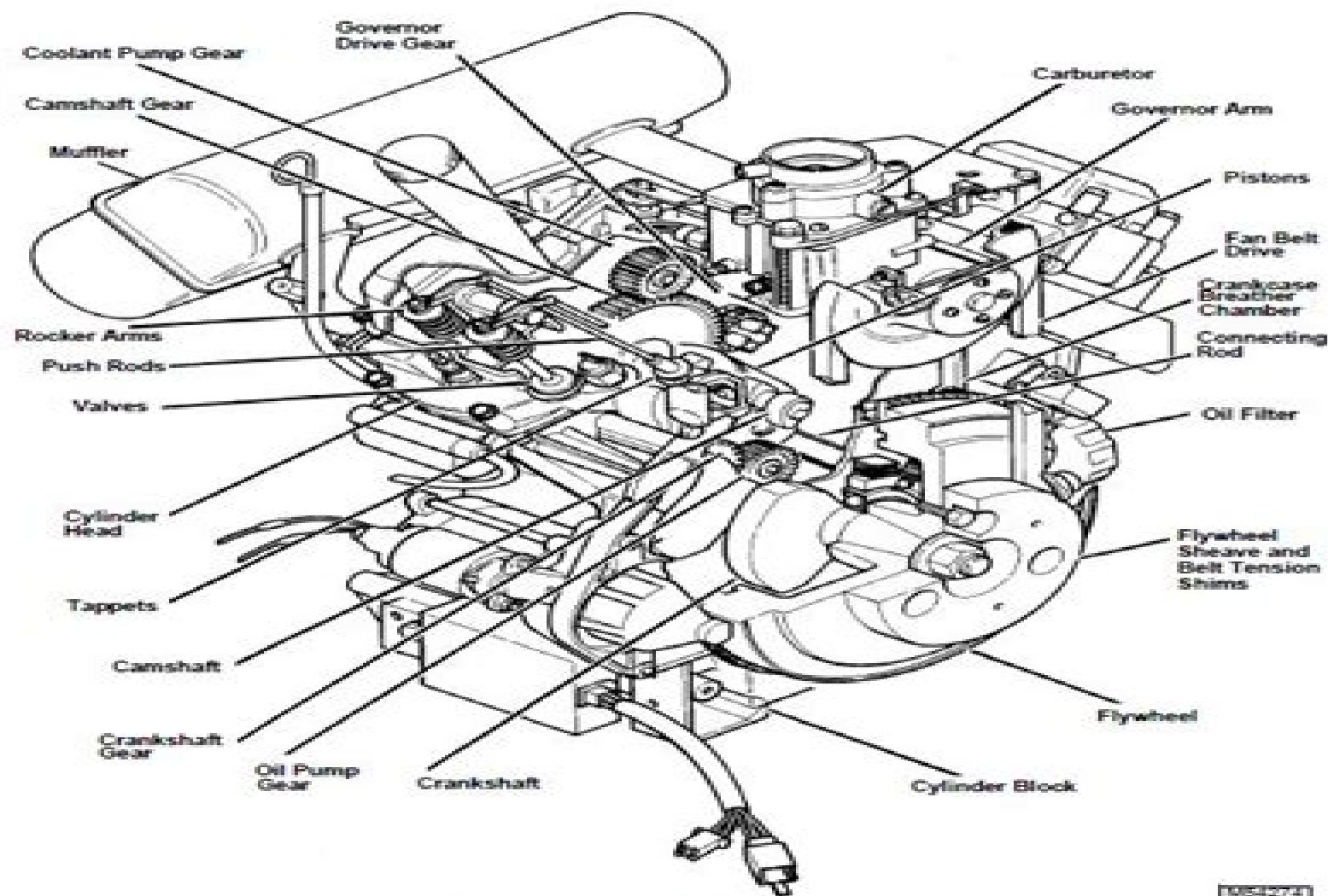
Cutaway—FD620D
