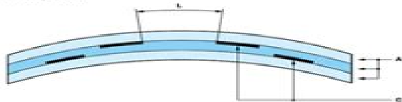
Figure 2. Diagram detailing clearance and creepage distance requirements for thin-film insulation.
