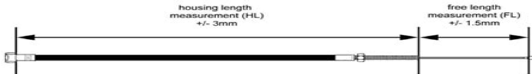
Clutch Cable Sample 2
