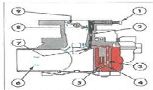
Figure 3 Idle System
